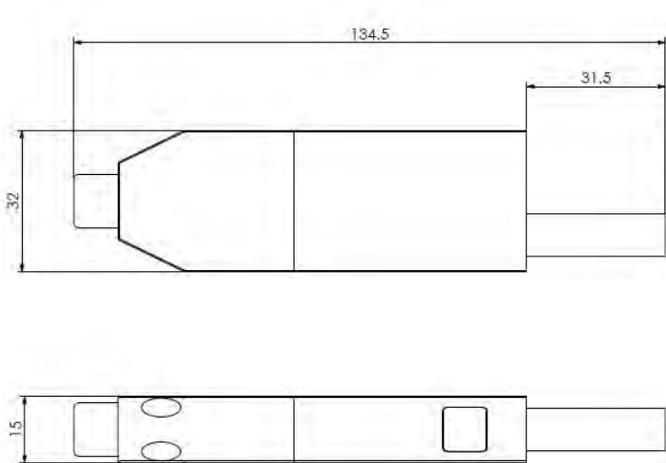
图 1 The size of with the protect shell. The 31.5mm stainless steel probe can be customized to any long (longer, shorter or 90° bend).
