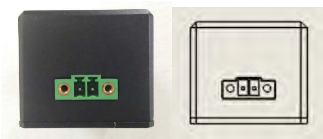
Fig 5.08-2P interface sketch
